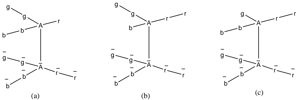
Figure 11. Structures of Down Antiquarks: (a); (b); and (c) are down antiquarks with different color charges
