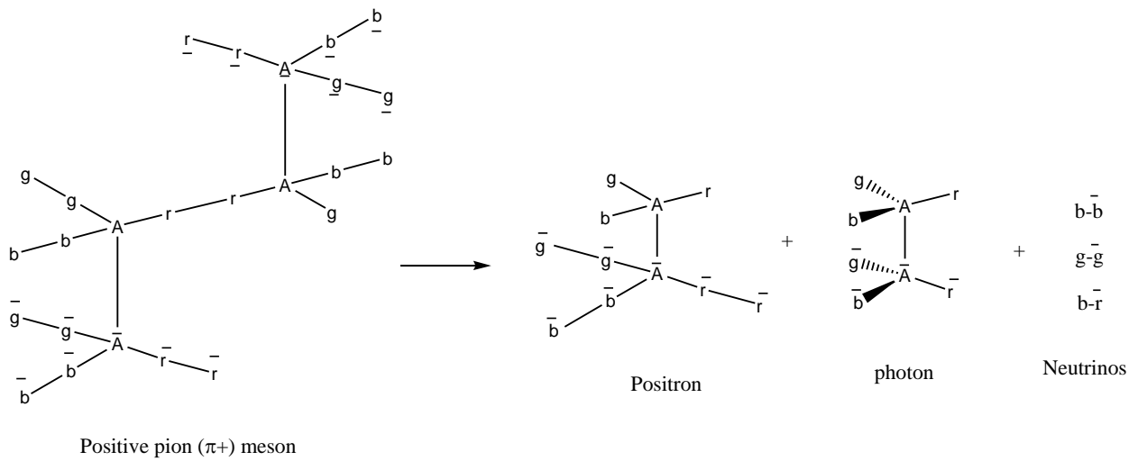
Figure 25. Positive pion ( \pi^+ ) mesons with a positive Charge Made from Up Quark and down Antiquark with Missed c-particles and Anti Particles and Decay
