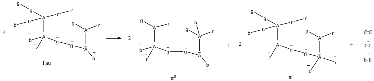
Figure 22. Tau Decay
