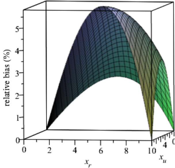
Figure 3: Example plot of the bias function with variables x_r, x_u ( T_u=30, T_{sub}=25, T_r=22, x_m=10 ). The maximum value is observed for x_u = x_r = 5.77
