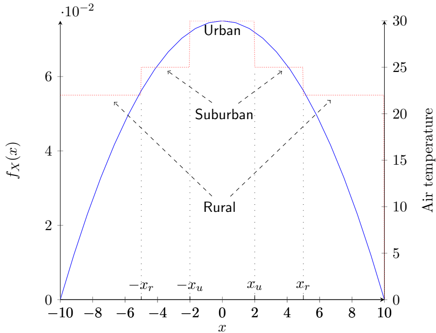
Figure 2: Plot of the pdf of the one-dimensional RWP model ( x_m=10 ), together with a simple model of an UHI (red densely dotted line).
