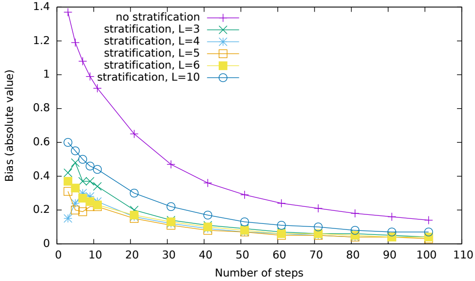
Figure 7: Absolute values of the bias with and without stratification for increasing number of steps of the environmental parameter function ( n = 20 , r = 0.7 , T_{min} = 22 , T_{max} = 30 )
