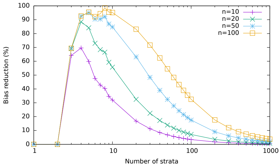
Figure 4: Bias reduction of the stratification method when weighting proportionally to stratum areas. The 3-step function shown in Fig. 2 is used for the environmental parameter.
