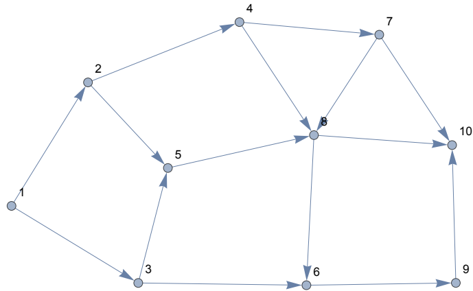
Figure 1: A 2-scale consisting of ten points. The straight lines denote the neighborhood structure.
