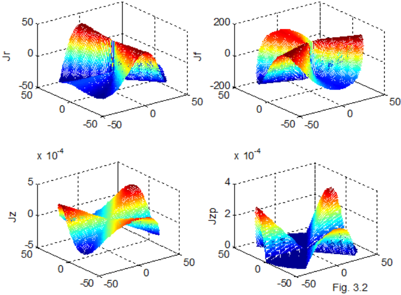
Fig. 3.2 illustrates functions (12-14), when z = const . The fourth window shows function
