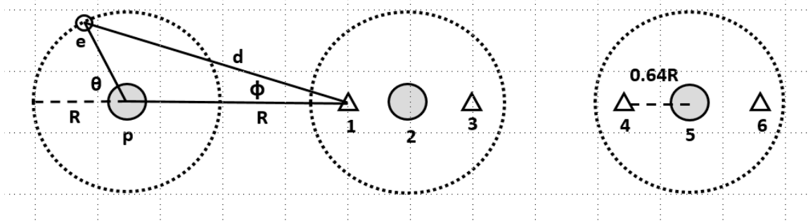
FIGURE 2. Geometric Arrangement of Three Hydrogen Atoms
