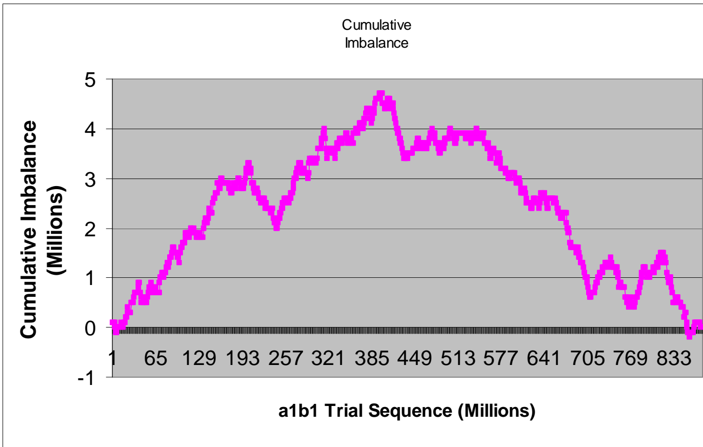
Figure 1 – Indication that the accumulation of imbalance has an overall direction till it reaches a peak and reverses the direction at the peak. Peak is at ~414 Million trials. Peak of cumulative imbalance is 4.7 million. A ++ appears to place peak at the ~middle of the graph (actual at 47% of total interval). Above zero count = 136644, below zero count = 4795, i.e. above zero = 96.6% of time.
