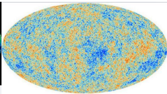
"Planck"-created map of the cosmic microwave background.
