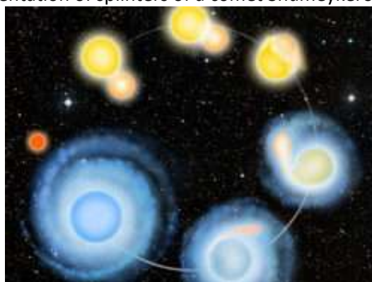
Fig. 3. Polarization of a congestion of galaxies
