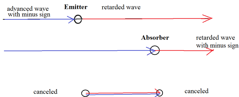
Figure 0. The Wheeler and Feynman model. The emitter sends retarded wave to right show as red arrow. The emitter sends advanced wave to the left which is blue. We have drawn the arrow in the opposite direction to the advanced wave. This is same to the absorber. However the retarded wave of the absorber is just the negative value of the retarded wave (or it has 180 degree phase difference). The advanced wave sent by the emitter is also with negative value of that of the absorber (or has 180 degree
