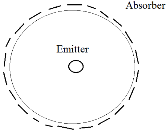
Figure 5. This shows emitters all at the center of the sphere. The absorbers are distributed at the surface of the sphere. The absorber is the environment. We assume the absorbers are surrounded the emitter. This is our simplified macrocosm model.
