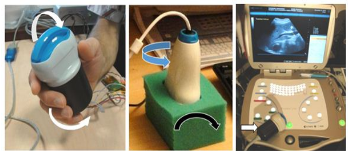
Figure 1: (a) Motorized probe (400cm 3 and 430g). The transducer (3,5MHz curved array) can be remotely tilted and rotated (arrows) from away by the expert while manipulating (b) the dummy probe (arrow) (c) the tele-operated portable Echograph(6kg) and tele-operated probe (arrow).
