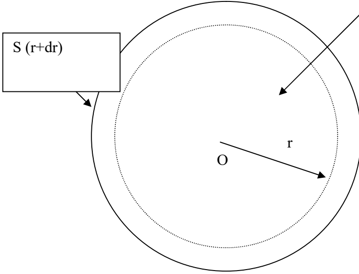
Figure 1: The spherical concentration of dark substance
