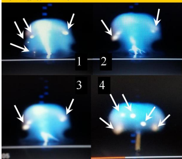
Figure 3, Microscopic Black Holes on Earth.
