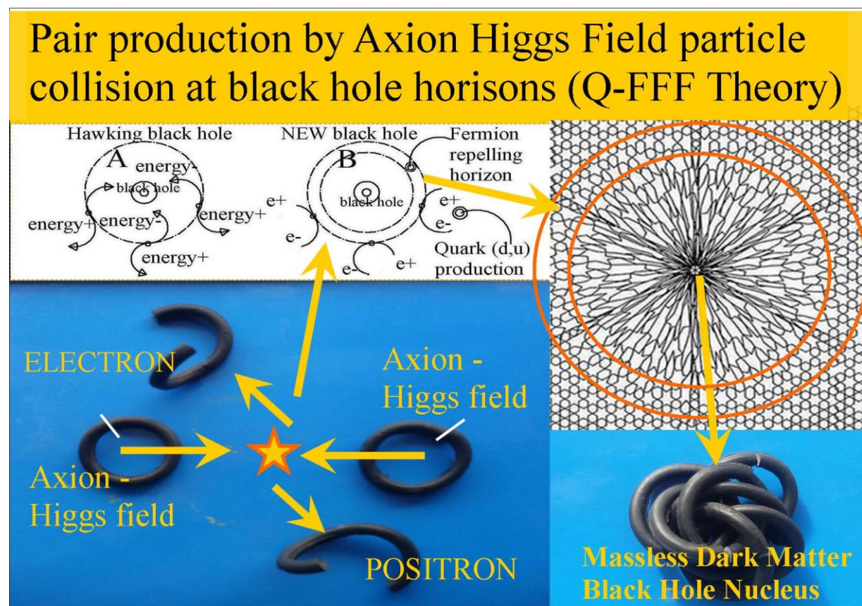
Figure 1. Pair production by Axion Higgs Field particle collision at black hole horizons (Q-FFF Theory)
