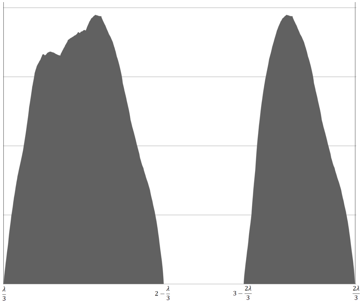
Figure 1 distribution of Ulam residues modulo \lambda
