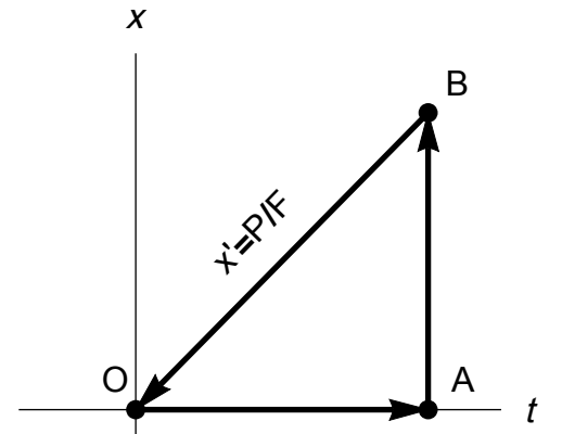
Figure 3.1: A "thermodynamic cycle" through space and time.
