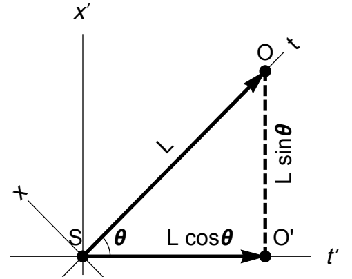
Figure 3.2: The space-time intervals between two observers. Here O' travels at speed |v| in O 's reference frame.
