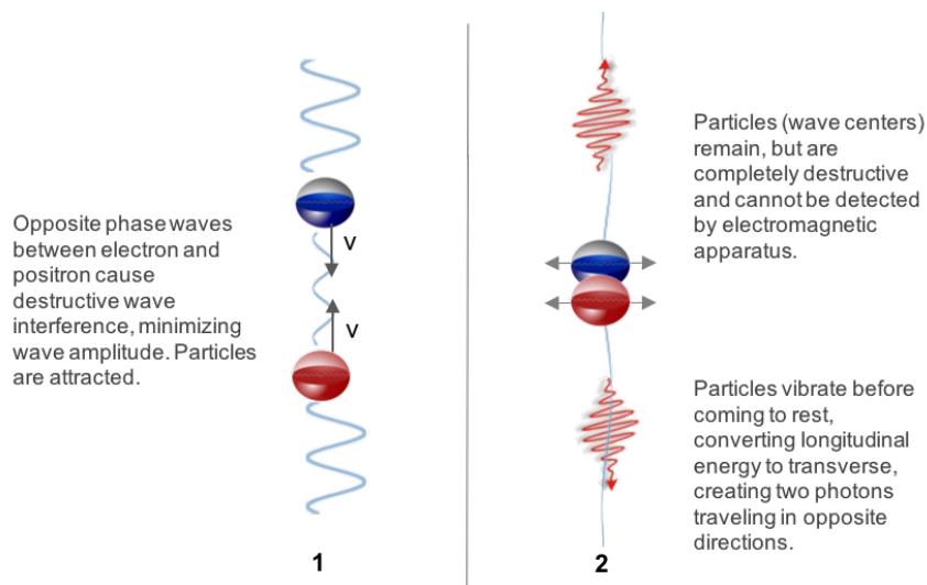
Fig 2.3 – Annihilation of Electron and Positron.
