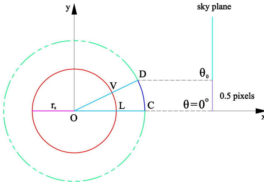
Figure 8 – Section in the xy plane of the outburst source (red circle) and of the sphere during its superluminal expansion (green dashed line). The angular aperture of the central pixel has been exaggerated for clarity purposes.
