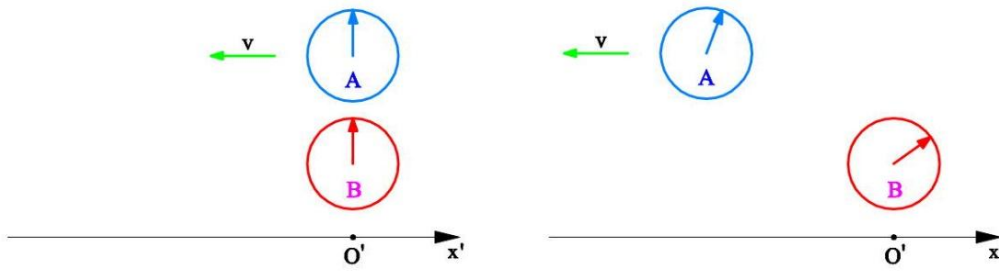
Figure 12 – Clock B at rest in the origin O' of the inertial reference frame R' and clock A moving along the x' axis at constant speed -v . The reading of the two clocks when superimposed in the origin is zero.
