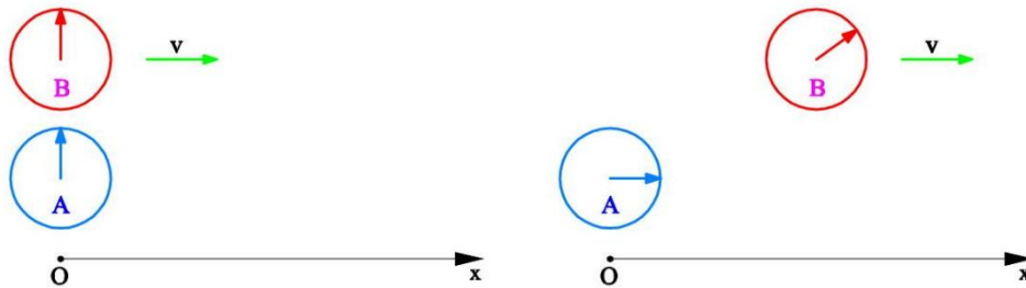
Figure 11 – Clock A at rest in the origin O of the inertial reference frame R and clock B moving along the x axis at constant speed v. The reading of the two clocks when superimposed in the origin is zero.
