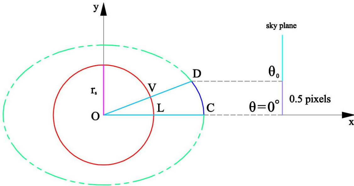
Figure 6 – Section in the xy plane of the outburst source (red circle) and of the deformed sphere resulting from optical illusion (green dashed line). The angular aperture of the central pixel has been exaggerated for clarity purposes.
