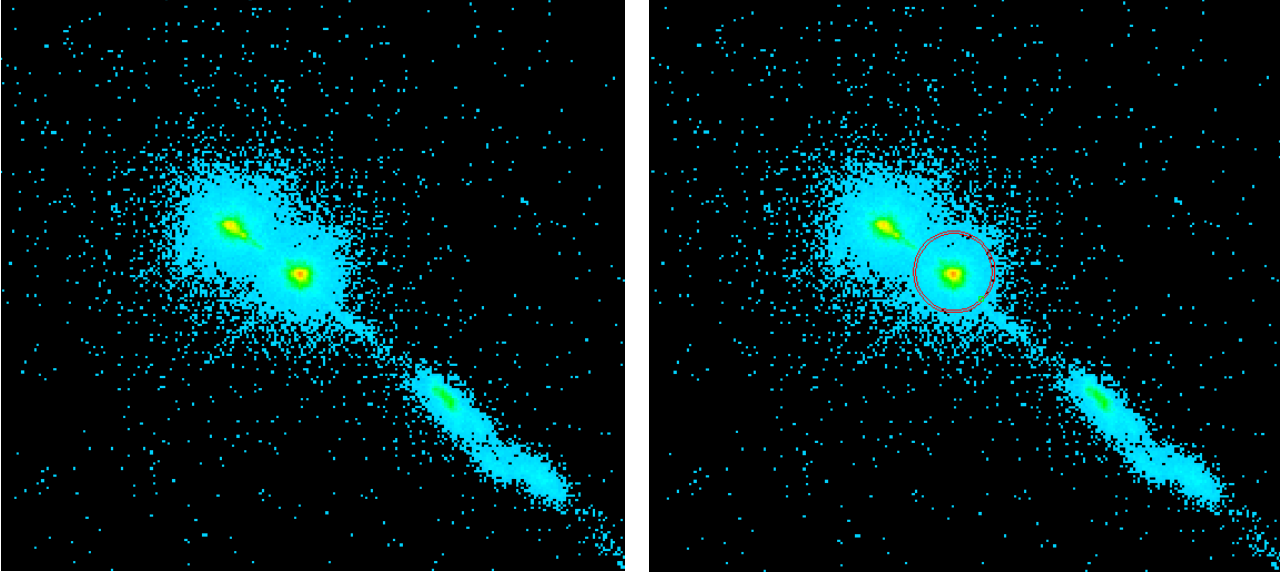
Figure 4 – Image from file o6n712tiqflt.fits of the HST-1 knot in 2003 July 27. The red annulus superimposed on the image on the right has an outer radius of 16.5 pixels and a thickness of 1 pixel (see later in the text).
