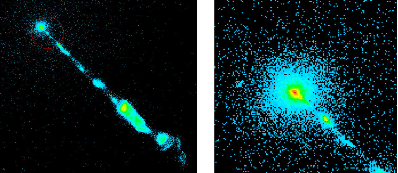
Figure 2 – Image from file o5dc01byq_flt.fits of the M87 jet (left) and a zoom of the HST-1 knot next to the AGN (right) in 1999 May 17. The meaning of the red circles superimposed on the images will be explained later in the text.
