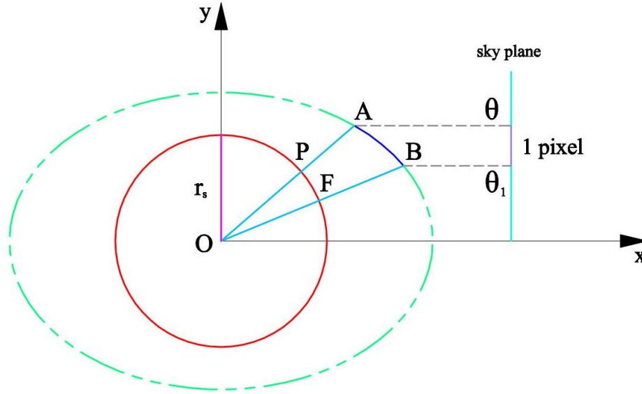
Figure 5 – Section in the xy plane of the outburst source (red circle) and of the deformed sphere resulting from optical illusion (green dashed line). The figure is symmetric around the x axis oriented along the direction of the line of sight OT .
