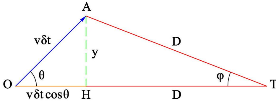
Figure 1 – Distance travelled by two light rays emitted from bright matter with time separation \delta t .
