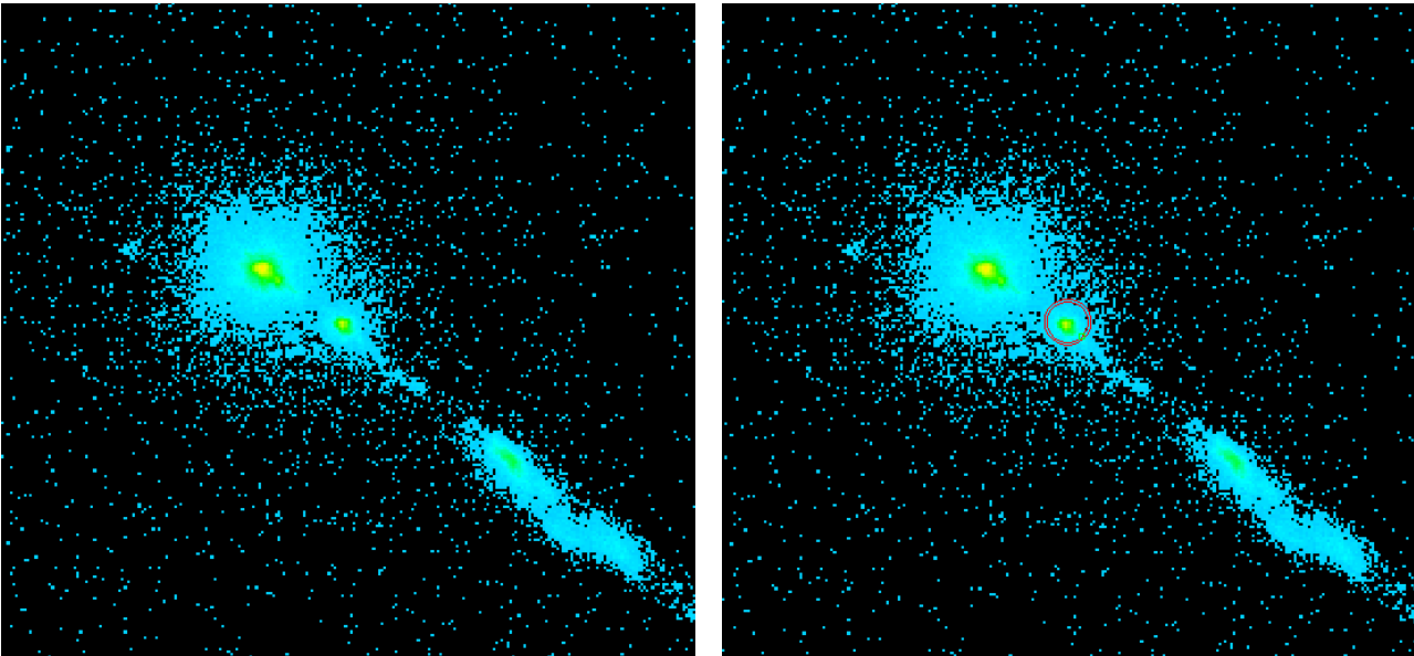
Figure 3 – Image from file o6a351evq_flt.fits of the HST-1 knot in 2001 July 30. The red annulus superimposed on the image on the right has an outer radius of 8.25 pixels and a thickness of 1 pixel (see later in the text).
