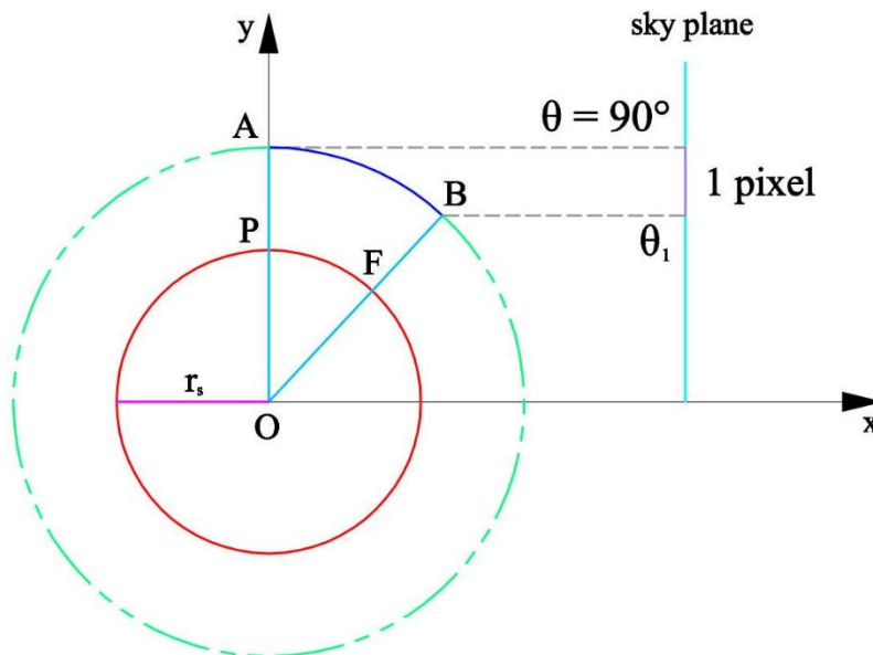
Figure 7 – Section in the xy plane of the outburst source (red circle) and of the sphere resulting from the expansion caused by the explosion process (green dashed line). The figure is symmetric around the x axis oriented along the direction of the line of sight OT.
