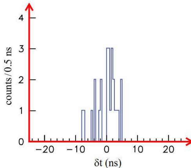
Figure 9 – Distribution for \delta t = \text{tof}_c - \text{tof}_v of the 25 events in ICARUS T600.
