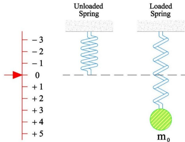
Figure 10 – Measurement of the rest mass m_0 by the stretching of a loaded spring.
