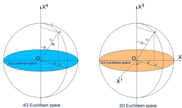
Figure 4: The generalized spherical coordinates \eta, \psi, \theta, \phi of 4-dimensional Euclidean space explained. Left panel: the radial coordinate \eta , and “polar” angle \psi . The blue plane represents the 3-dimensional hyper-plane normal to the x_4 axis. The other two coordinates of the point A are the same as the coordinates of projected point A' in this hyper-plane. Right panel: the spherical coordinates of point A' in the hyper-plane. (Diagram modified from Figure3.1 in [5])
