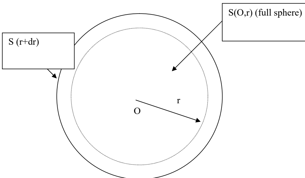
Figure 1: The spherical concentration of dark substance
