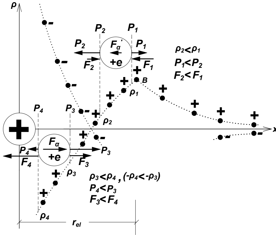
Figure 5. In the lower inverse nuclear field, which has negative units in abundance, an increase the magnetic dipole moment of neutron and proton and a repulsive antigravity force 13,14 F_\alpha are created
