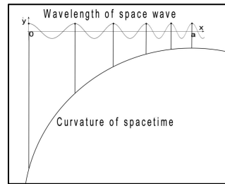
FIG. 7. The spacetime curvature can be transformed into a Space wave as gravity. There is a new theory growing out of the general theory of relativity holding its values. This new theory is the Space-Matter Theory.
