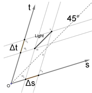
FIG. 2. The speed of light in the Minkowski geometry. t is time in meters, c = 1 , and s is the spatial distance in meters. \Delta s / \Delta t = 1 = c . (According to my opinion, this unit is the real unit that matter uses, since t and s comes from the space waves. See later.)
