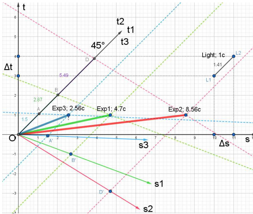
FIG. 11. All three experiments of tunneling are shown here. t (=tc) and s are in meters. In our coordinate system st (or in light's space) the unit is given by light with this function:
