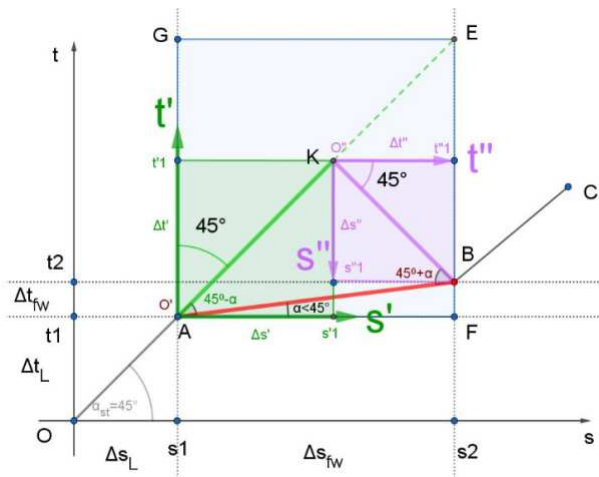
FIG. 14. Time and spatial distance are in meters. The figure shows how to put a fast wave into
