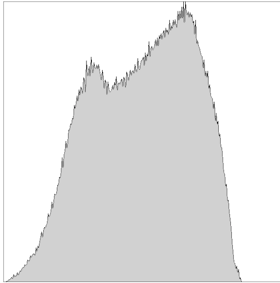
Figure 3: Displacements of Z' = Z^2 + C , where C_{xyzw} = 0.3, 0.5, 0.4, 0.2 . For this histogram the maximum displacement is 2.36506. Mean: 1.38231; standard deviation: 0.496788; variance: 0.246798; skewness: -0.214489 ; kurtosis: -0.933944 ; peak value: 1.53986.
