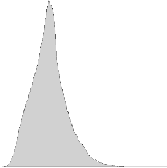
Figure 2: Lengths of Z' = Z^2 + C , where C_{xyzw} = 0.3, 0.5, 0.4, 0.2 . For this histogram the maximum length is 21.2391. Mean: 7.05497; standard deviation: 2.58653; variance: 6.69016; skewness: 0.506456; kurtosis: 0.643926; peak value: 5.95688.
