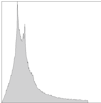
Figure 4: Magnitudes of Z' = Z^2 + C , where C_{xyzw} = 0.3, 0.5, 0.4, 0.2 . For this histogram the maximum magnitude is 3.99997; mean: 1.18208; mode 0.614353.
