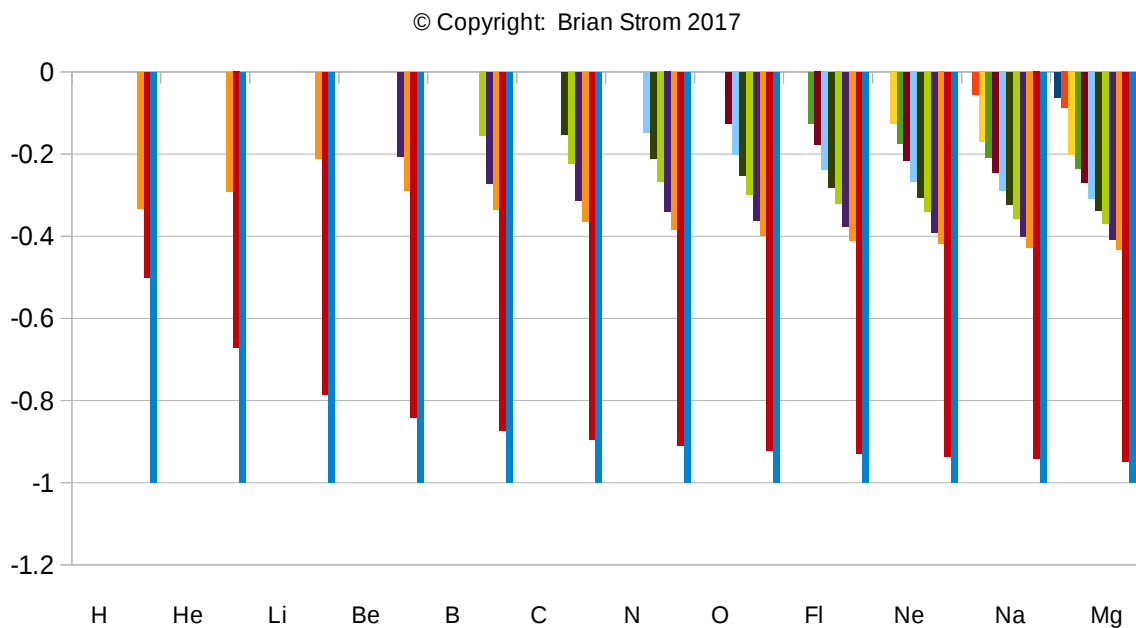
Figure 5b. IONIZATION: Histogram of electron depths per proton – normalized.
