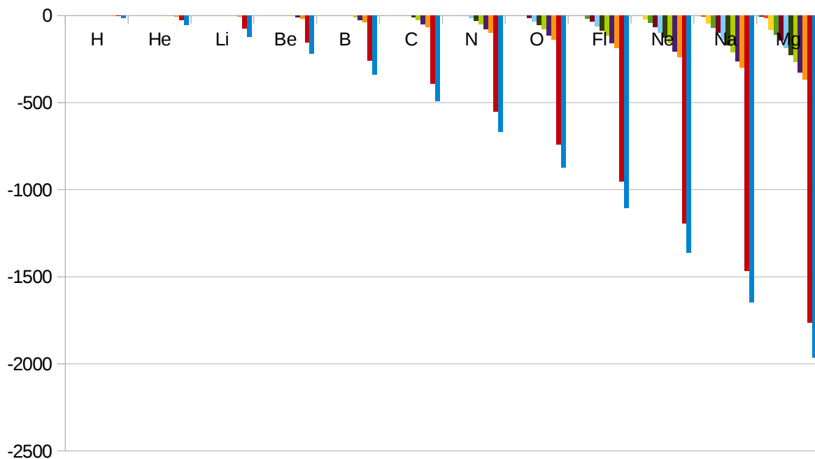
Figure 2b. IONIZATION - Histogram of energies to remove electrons.
