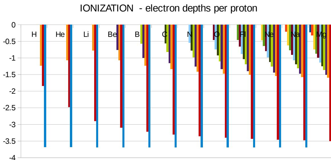
Figure 4b. IONIZATION: Histogram of electron depths per proton.
