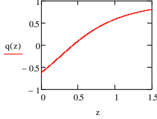
Figure 1. Re-acceleration of the universe based on Beckwith [6] ; (note that q(z) < 0 if z < .423 ).
