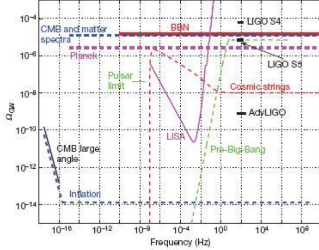
Figure 1. Abbott et al.[14] (2009) shows the relation between GW frequency and GW energy density for different cosmological models
