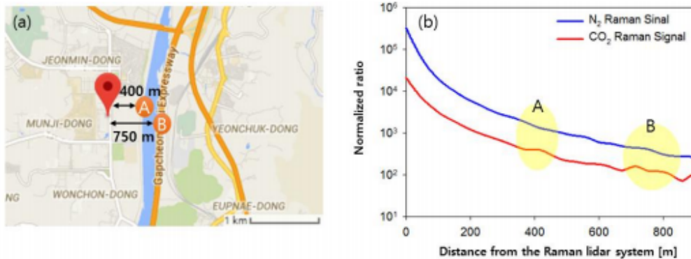
Figure 6. (a) Study area in Daejeon, Korea; (b) N 2 and CO 2 Raman signals measured by the Raman lidar system.
