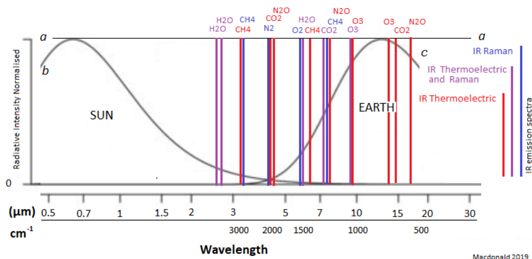
Figure 53. Quantum Predicted IR Spectra with Sun and 'Earth Blackbody' Curves. Spectrogram shows positions and type of the predicted IR emission spectra of gas molecules within the EMS
