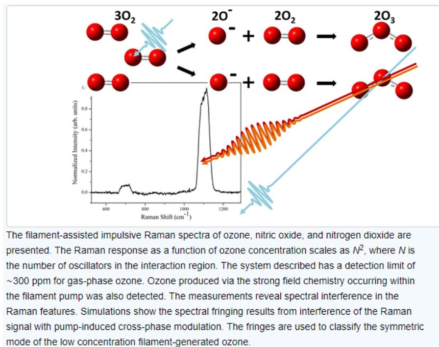
Figure 49. O 3 Raman Spectrograph Showing its 1103cm -1 [75]
