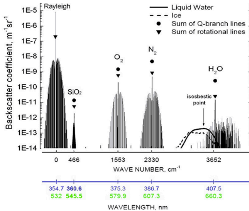
Figure 35. Showing N 2 O 2 H 2 O with Raman Number 112]
