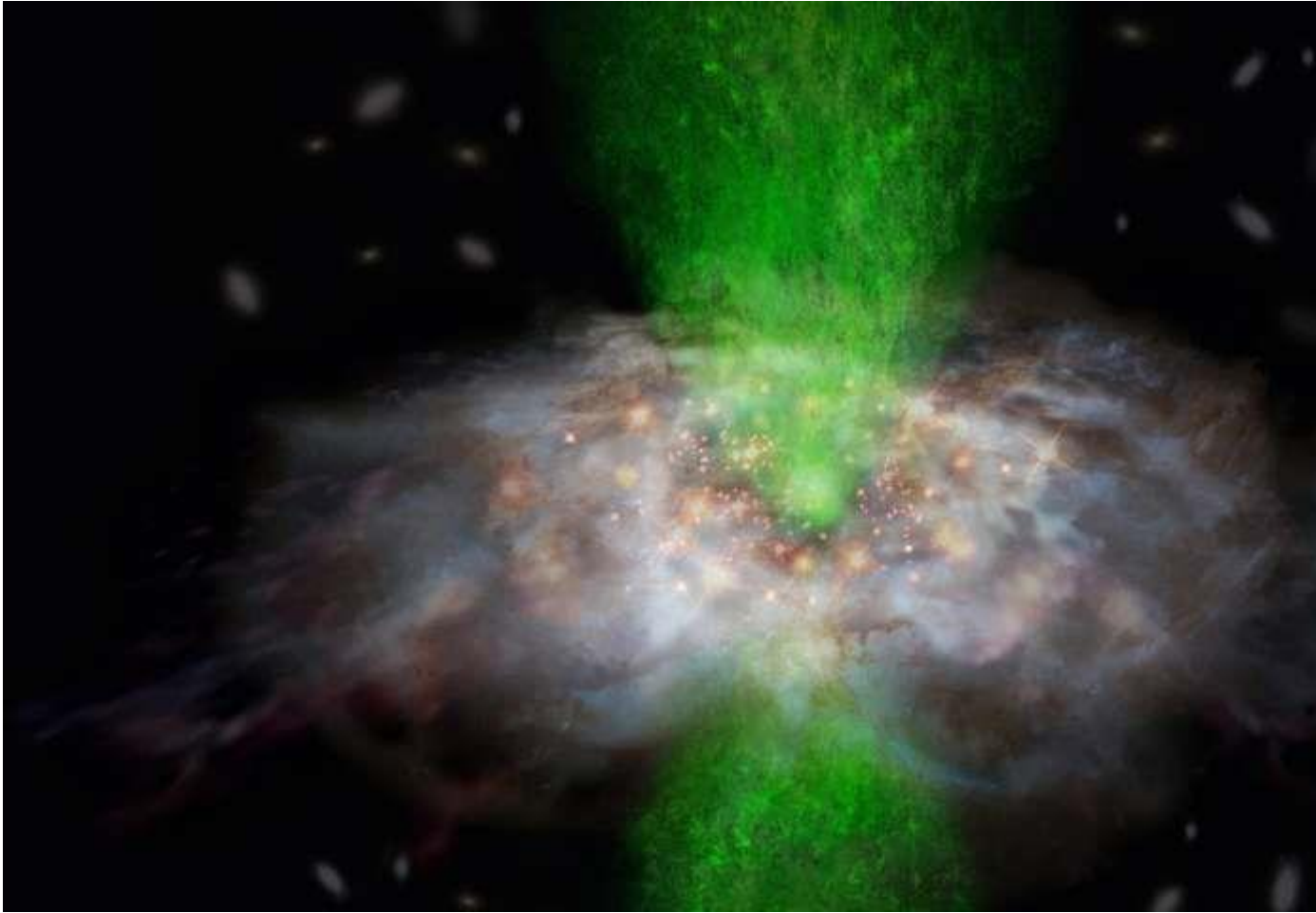
Figure 3: A schematic view of the fact that an ionized gas outflow (green) driven by the central supermassive black hole does not affect the star formation of its host galaxy. This situation may occur if the ionized gas is outflowing ...more
