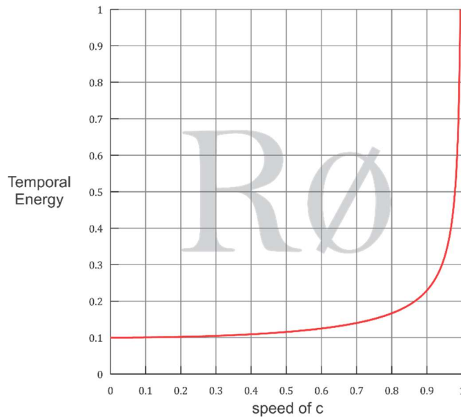
Figure 2. R0 (r-naught)
