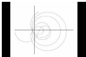
Fig. 3 OUTPUT for \sigma = \frac{2}{5} .
