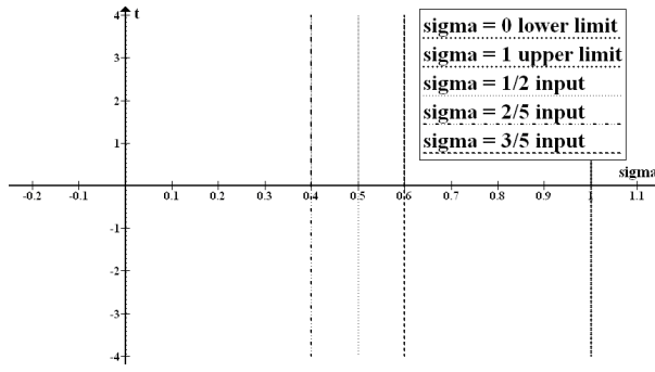
Fig. 1 INPUT for \sigma = \frac{1}{2}, \frac{2}{5}, and \frac{3}{5} . \zeta(s) has CIS of Completely Predictable trivial zeros at \sigma = all negative even numbers and CIS of Incompletely Predictable nontrivial zeros at \sigma = \frac{1}{2} for various t values.
