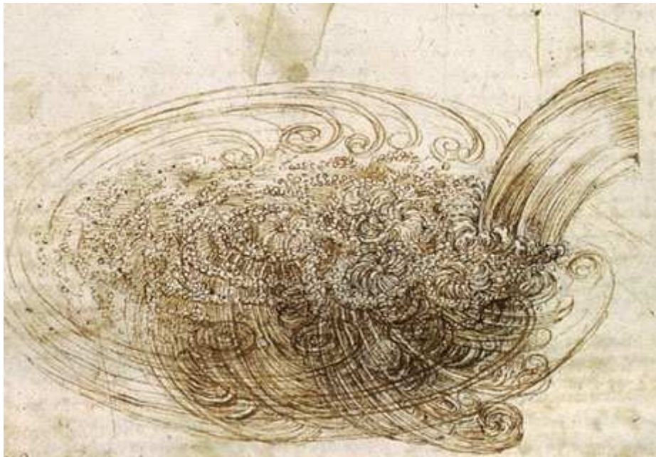
Figure 3.1.: Turbulences understood by Leonardo da Vinci
