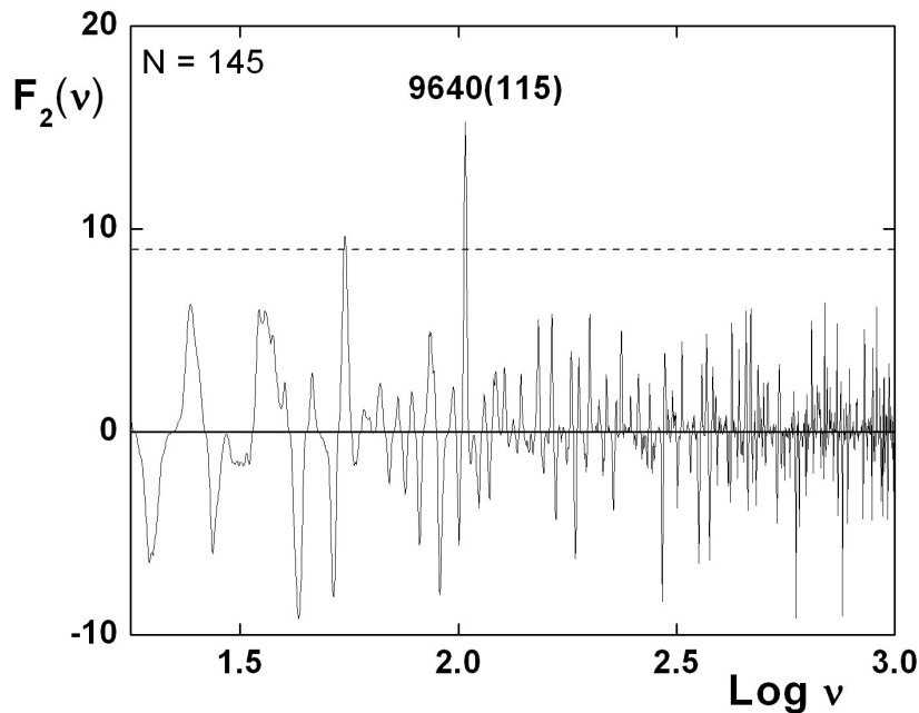
Figure 5. Same as Fig. 4, for the F_2(\nu) spectrum, computed for N = 145 exoplanets with P < 1.5 days. The strongest peak of the composite commensurability corresponds to a period of 9640(115) s at nearly 3.9\sigma significance (after Kotov, 2018).
