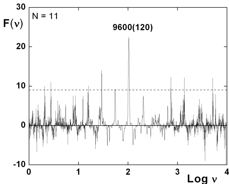
Figure 3. Same as Fig. 2, for N = 11 sizes («diameters») of the solar system (with c = 1 and the \pi factor for inner orbits). The highest peak corresponds to the spatial scale 9600(120) light sec.
