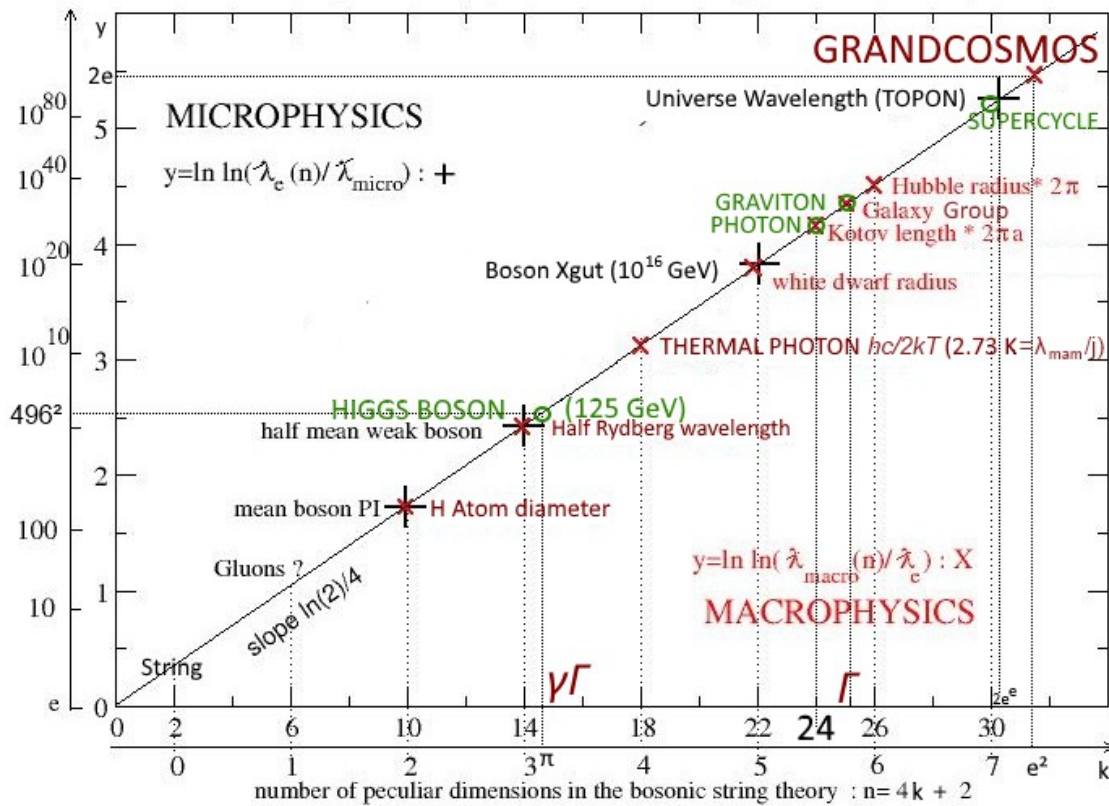
Figure 1. TOPOLOGICAL AXIS [3]. Double logarithm ( y = \ln(\ln Y) ) of main dimensionless quantities Y corresponds to the String dimension series n = 4k + 2 , from k = 0 to 7 , showing the Cartan-Bott periodicity \Delta n = 8 [25], which is at the origin of the name 'Topological Axis'.
