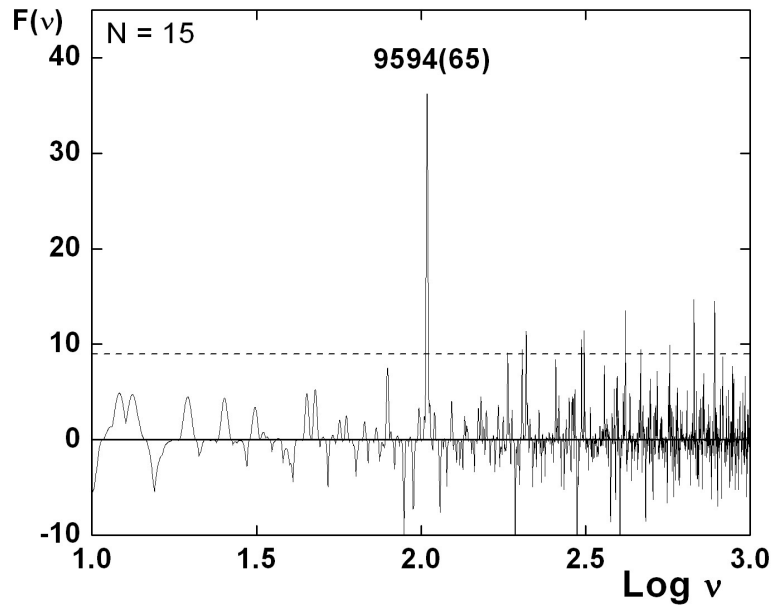
Figure 2. Resonance-spectrum F(\nu) computed for 15 motions of the largest, fast-spinning bodies of the solar system. On horizontal axis is logarithm of frequency \nu (in \mu\text{Hz} ), the dashed horizontal line shows a 3\sigma C.L., and the primary peak corresponds to the best-commensurable period 9594(65) s.
