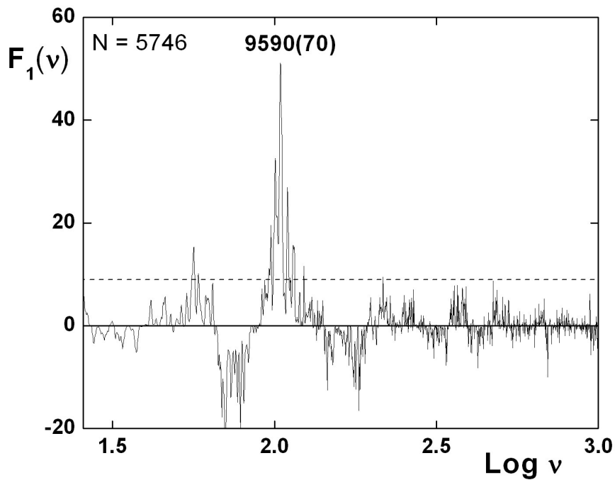
Figure 4. Resonance-spectrum F_1(\nu) , computed for N = 5746 binaries with periods < 5 days. Horizontal axis gives logarithm of the trial frequency \nu (in \mu\text{Hz} ), the dashed line indicates a 3\sigma C.L., and the major peak corresponds to a timescale of 9590(70) s.
