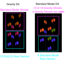
12 SU(2,2) Root Vectors 8 Standard Model Root Vectors
