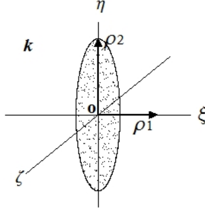
Fig. 4: The radius \rho_2 = c\tau of the expanding light-circle in the \eta - \zeta plane (shaded area) is not the same as \rho_1 = c\tau of the light wavefront on the \xi -axis in the direction of motion v , because the respective times \tau are not the same since time depends upon position \xi in system k under Lorentz Transformation from system K .
