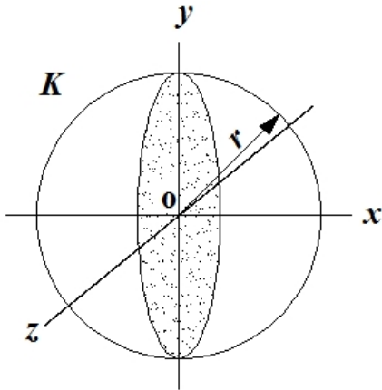
Fig. 1: After a time t > 0 a sphere of light of radius r = ct expands in inertial system K . All positions on the x -axis within the sphere record the same time t and the same radius r = ct . The expanding great circle of light in the y - z plane (shaded area) has the same radius as the wavefront on the x -axis.
