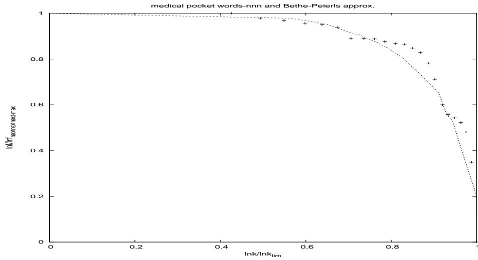
FIG. 37. Vertical axis is \frac{\ln f}{\ln f_{nextnextnext-max}} and horizontal axis is \frac{\ln k}{\ln k_{lim}} . The + points represent the words of the pocket medical dictionary with fit curve being Bethe-Peierls curve in presence of four nearest neighbours.
