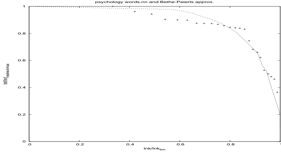
FIG. 24. Vertical axis is \frac{\ln f}{\ln f_{nextnext-max}} and horizontal axis is \frac{\ln k}{\ln k_{lim}} . The + points represent words of the psychology dictionary with fit curve being Bethe-Peierls curve with four nearest neighbours.
