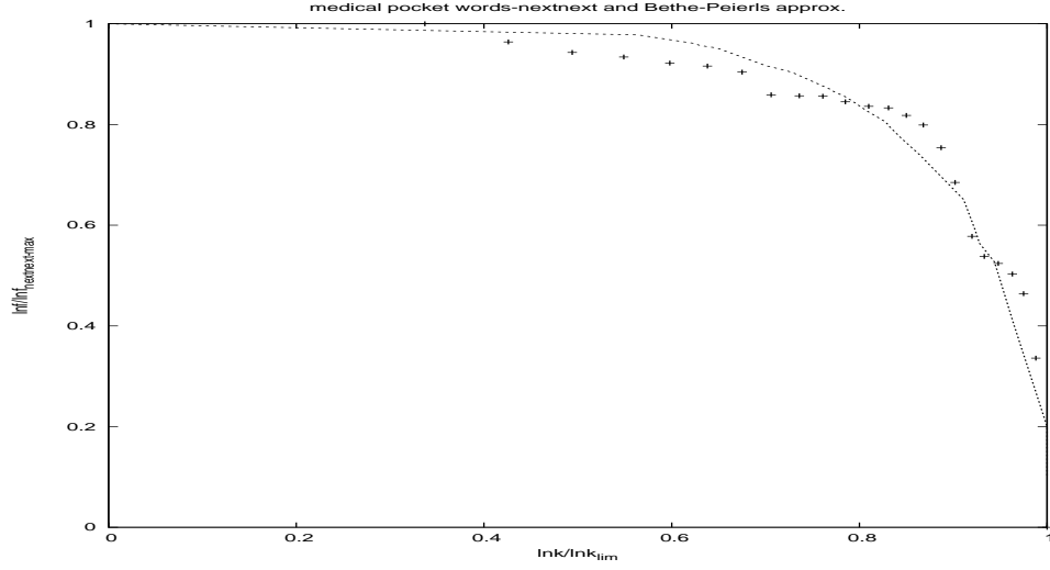
FIG. 36. Vertical axis is \frac{\ln f}{\ln f_{nextnext-max}} and horizontal axis is \frac{\ln k}{\ln k_{lim}} . The + points represent the words of the pocket medical dictionary with fit curve being Bethe-Peierls curve in presence of four nearest neighbours.
