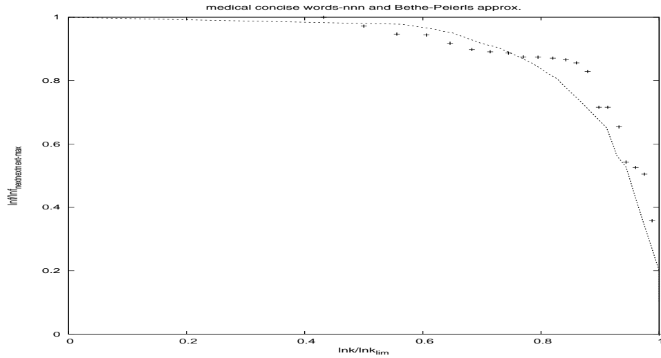
FIG. 31. Vertical axis is \frac{\ln f}{\ln f_{\text{nextnext-max}}} and horizontal axis is \frac{\ln k}{\ln k_{\text{lim}}} . The + points represent the words of the concise medical dictionary with fit curve being Bethe-Peierls curve in presence of four nearest neighbours.
