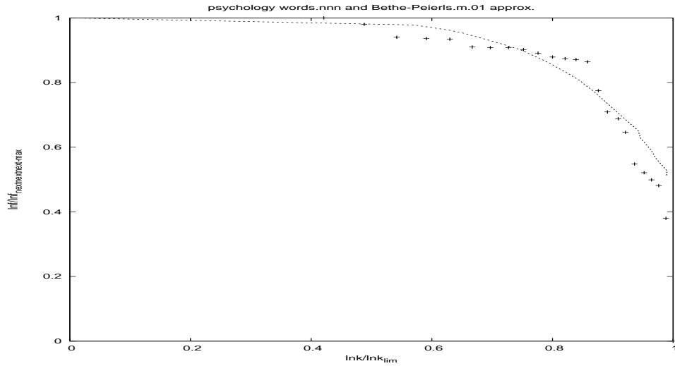
FIG. 25. Vertical axis is \frac{\ln f}{\ln f_{nextnextnext-max}} and horizontal axis is \frac{\ln k}{\ln k_{lim}} . The + points represent words of the psychology dictionary with fit curve being Bethe-Peierls curve in presence of four nearest neighbours and little magnetic field, m = 0.01 or, \beta H = 0.02 .
