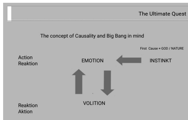
Picture 3.: Analog comparator with feedback-loop in brain
