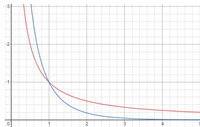
Figure 3: The Yukawa versus the Coulomb potential
