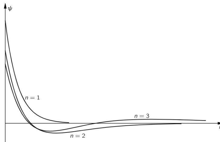
Figure 4: Wavefunction for electron s -states ( l = 0 ) 27
