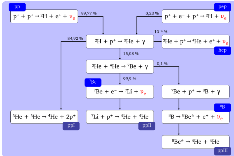
Figure 1: Nuclear reaction routes in the Sun
