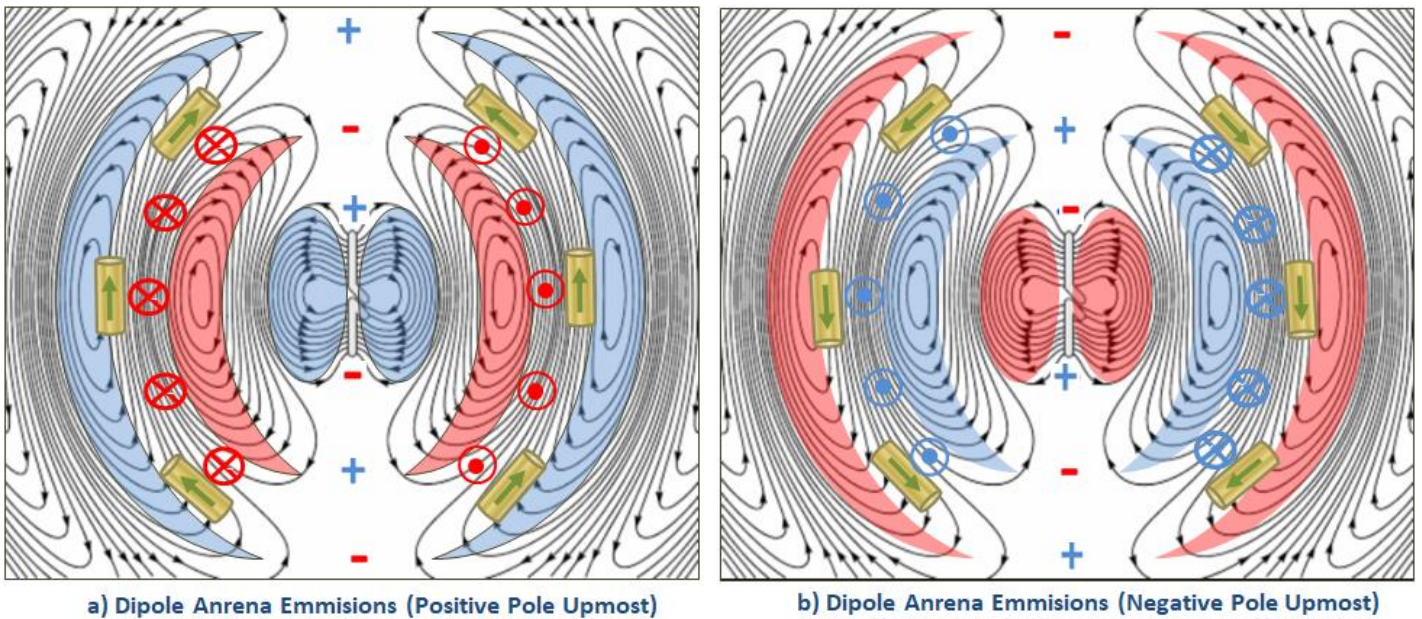
Figure 17: Radio Wave Electromagnetic Field Patterns for a Dipole Antenna
