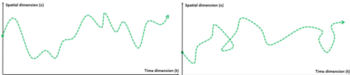
Figure 2: A well- and a not-well behaved trajectory in spacetime 20
