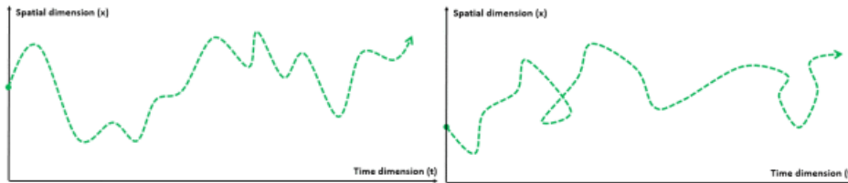
Figure 1: A well- and a not-well behaved trajectory in spacetime 12
