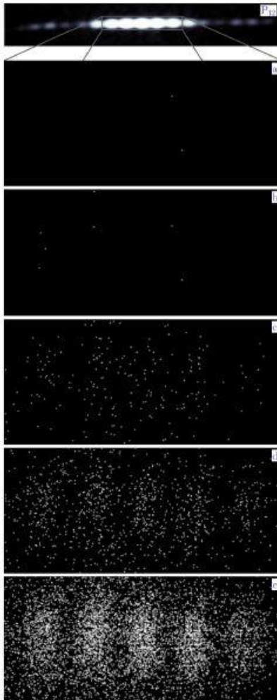
Figure 6: Diffraction and interference patterns (double-slit experiment with electrons) 84
