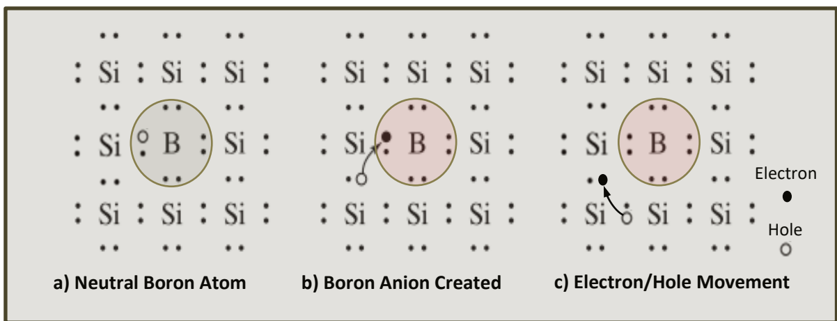
Figure 1: Electron/Hole Movement in p-type Semiconductor
