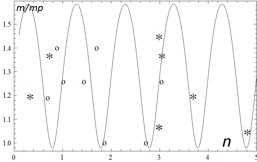
Figure 2: Comparison of baryons masses calculated from eq. (6) (line) as a function of confined flux n , with data points from Tables 1 and 2 of ref.[2] for octet ( open circles) and decuplet particles ( m_t used[2], stars). Nucleons are on the basis of the figure. The points come from the heuristic/phenomenological equation n = (2 c^2 \alpha / e^3) \mu m . The fit produces U_0 = 3710 MeV as the vacuum parent level.
