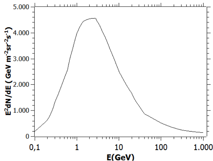
Figure 3: Interstellar energy-flux profile of protons in CR, which peak at, and have an average energy of 2.7 GeV kinetic energy[6].
