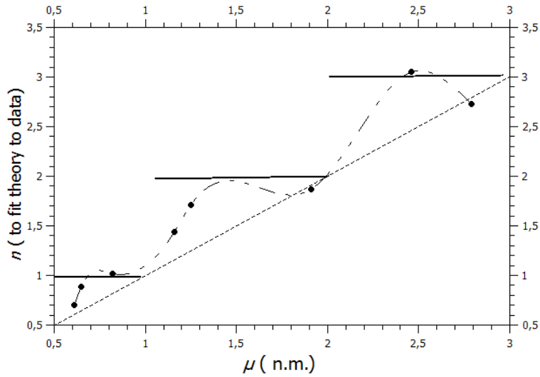
Figure1: Plot of n against the magnetic moment for the baryons octet ( points) from the definition n = (2 c^2 \alpha / e^3) \mu m . The diagonal line is the classical prediction of one flux quantum per nuclear magneton (n.m.). Nucleons are on the line. The data display undulations, and a tendency to reach for the steps ( traced line as guide)[2].
