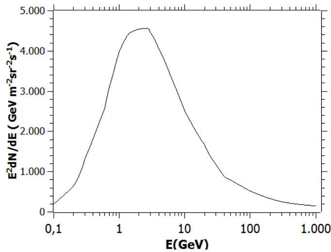
Figure 3: Interstellar energy-flux profile of protons in CR, which peak at, and have an average energy of 2.7 GeV kinetic energy[6].
