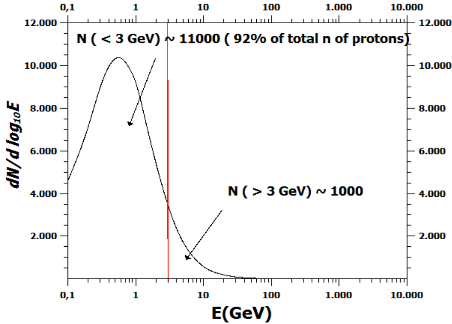
Figure 4: The previous figure is replotted to clearly show the concentration of protons below 3 GeV kinetic energies. The density peaks at 0.6 GeV, with protons reaching a relaxed configuration after radiating their excess energy.
