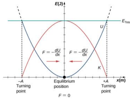
Figure 4: Kinetic (K) and potential energy (U) of an oscillator 46
