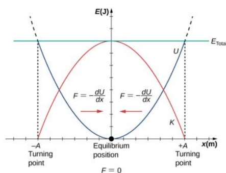
Figure 4: Kinetic (K) and potential energy (U) of an oscillator 47
