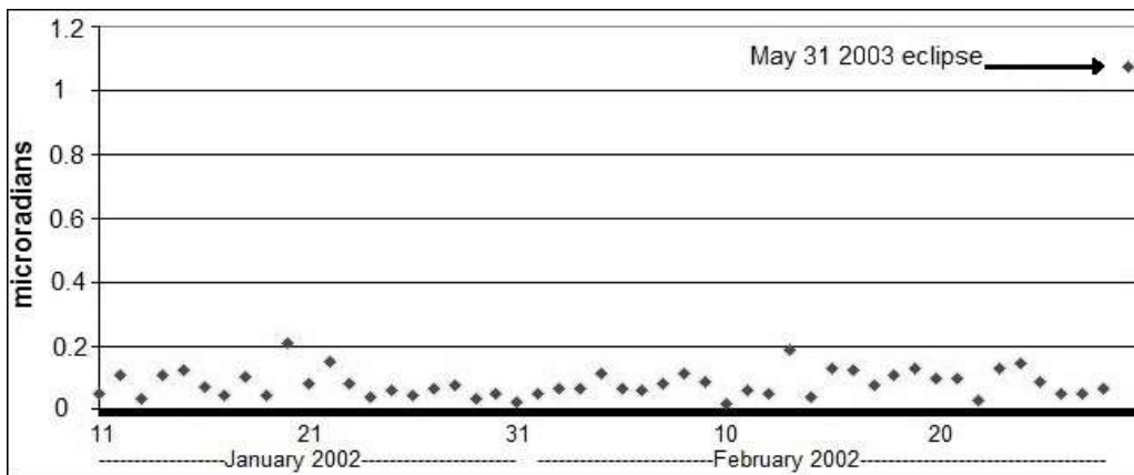
Fig. 10 – Dispersion of data in the control test and in the eclipse test. See text.
