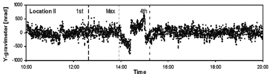
Fig. 17– Reported East-West tilt of the vertical during the March 29 2006, corrected
