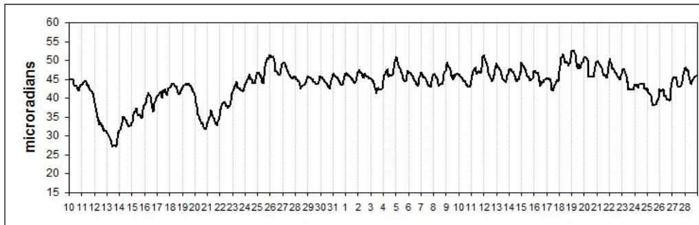
Fig. 4 – Same as Fig 3, but North-South. Top is South
