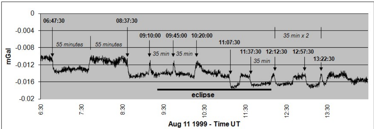
Fig. 21–The most relevant slice of the Trieste trace, with detailed timing info.
