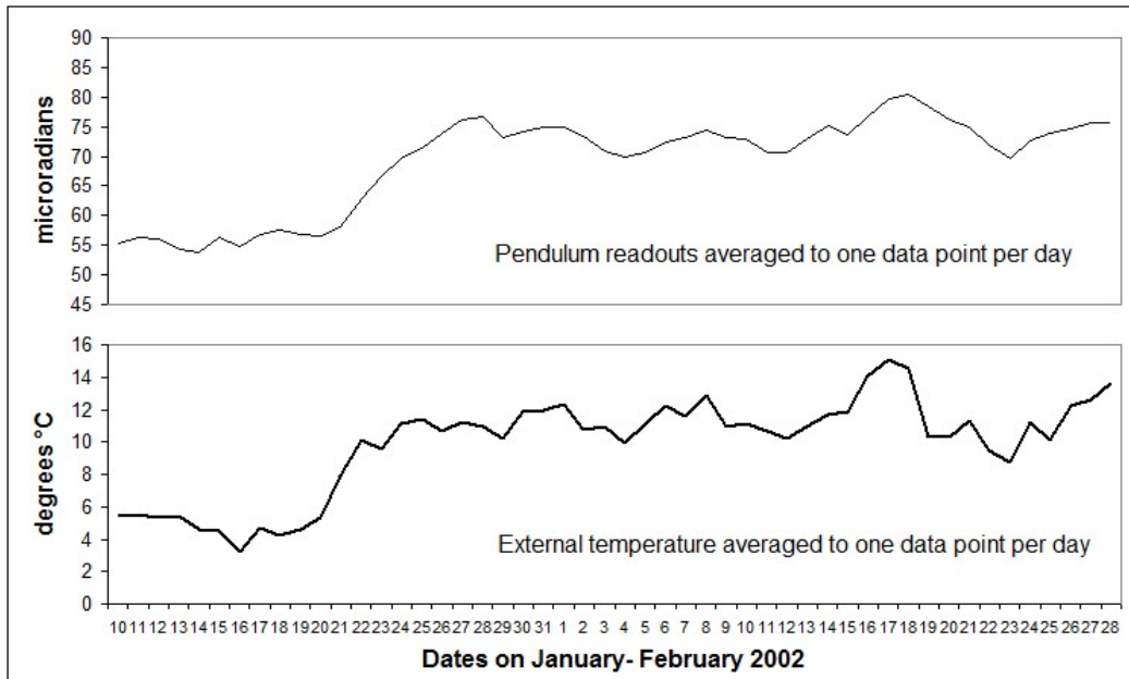
Fig. 5 – Correlation in the long term between pendulum readings and external temperature. Top is East
