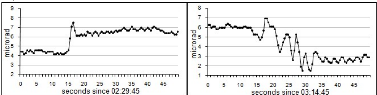
Fig. 15 – Details on the leading and trailing edges of the pulse at 02:30:00
