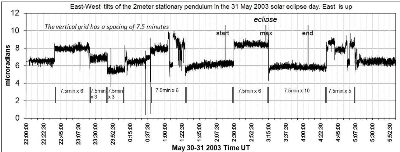
Fig. 12 – Temperature-corrected 8-hour continuous data around the eclipse. East-West
