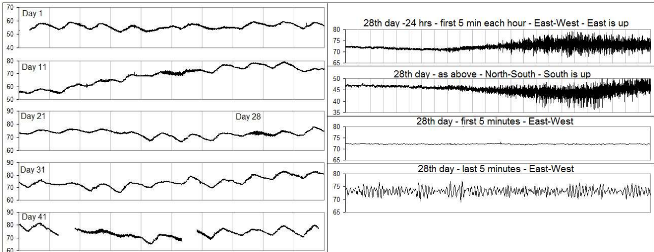
Fig. 7 – Left panel: the 50 days are charted in more detail, with data points averaged every 2.5 seconds. Right panel: the 28 th day raw data.
