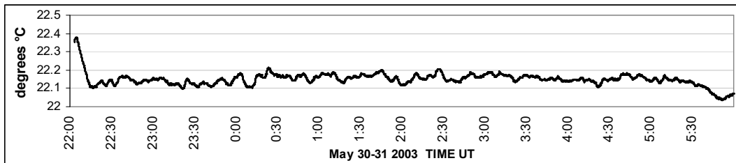
Fig. 13 – Temperature in the laboratory during the eclipse test
