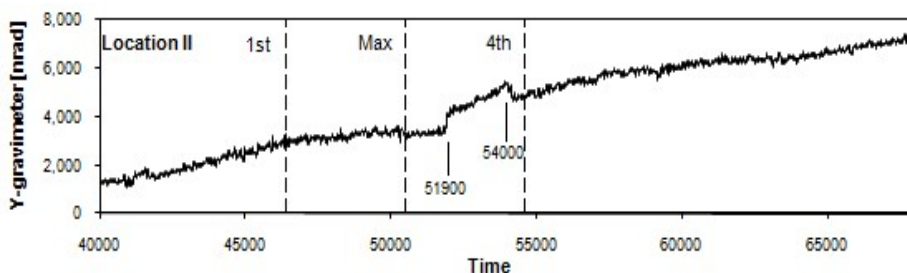
Fig. 18– Reported East-West tilt of the vertical during the March 29 2006, uncorrected. The time is seconds in the day. 51900=14:25:00, 54000=15:00:00 – Duration 35 minutes
