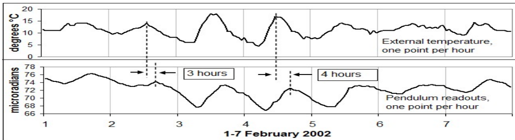
Fig. 6 – Correlation in the short term. Also seen the phase offset. Top is East
