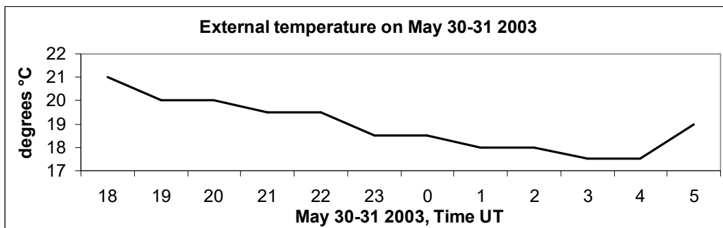
Fig. 14 – External temperature during the eclipse test plus the four previous hours
