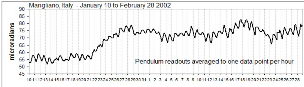
Fig. 3 – 50-day East-West pendulum oscillations relative to the tilting laboratory. Top is East
