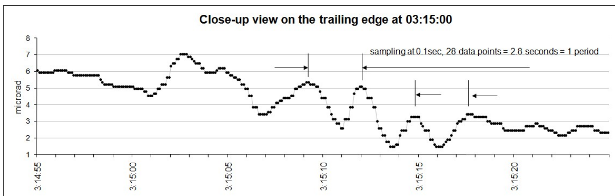
Fig. 16 – Close-up view on the 03:15:00 trailing edge
