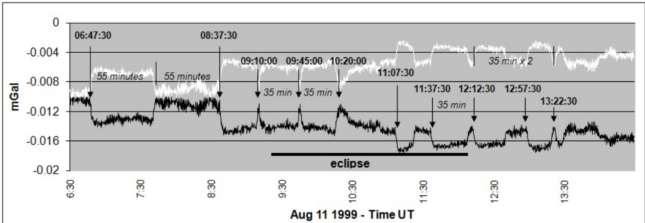
Fig. 23—Same as Fig. 21, but with mirrored trace added
