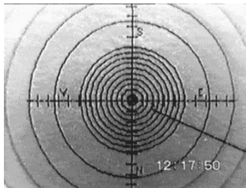
Fig. 19– Snapshot of the video permanently showing the bottom of pendulum #1.
