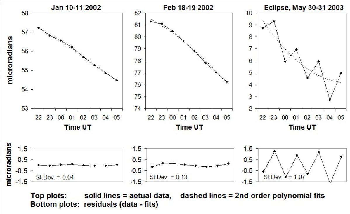
Fig. 9 – Graphic illustration of the data processing procedure. See text
