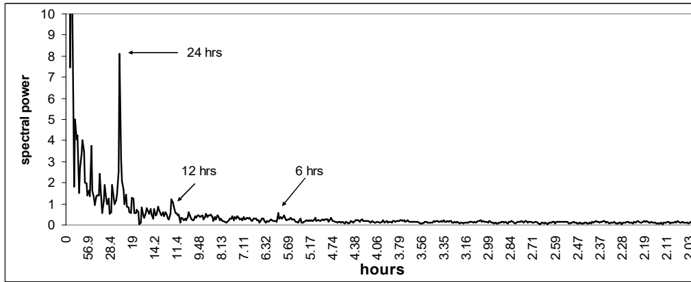
Fig. 8 – Fast Fourier Transform analysis of the data
