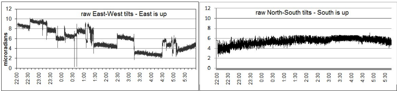
Fig. 11 – Uncorrected 8-hour continuous data around the eclipse.. East-West and North-South
