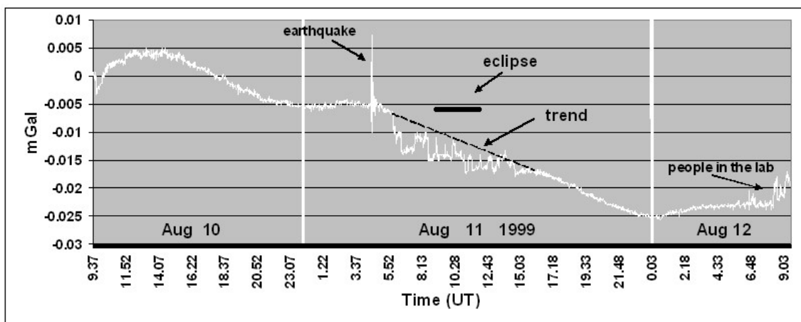
Fig. 20–Trieste gravimeter data at 90second resolution.
