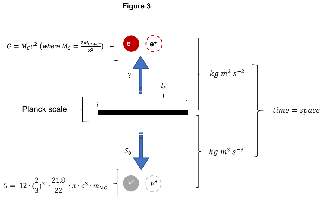
Figure 3 , highlighting the s (seconds) = m (metres), time = space , feature of the equations for G .
