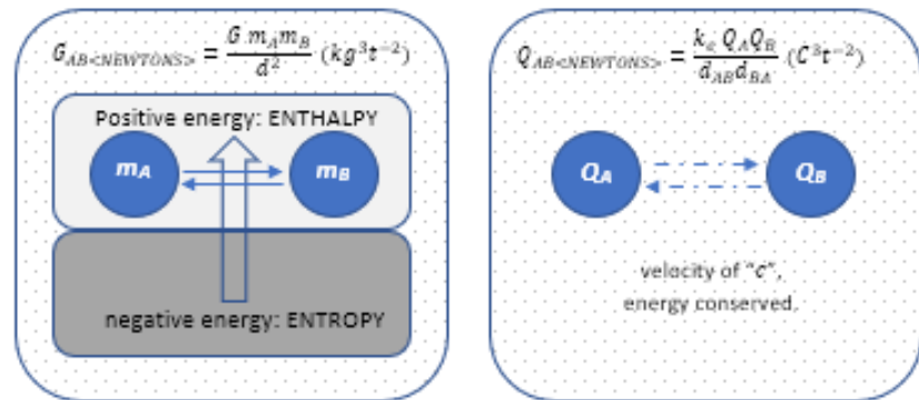
Paper 22, Figure 1: highlighting the difference of energy transfers in space in regard to G <m_A-m_B> and EM <Q_A-Q_B> .
