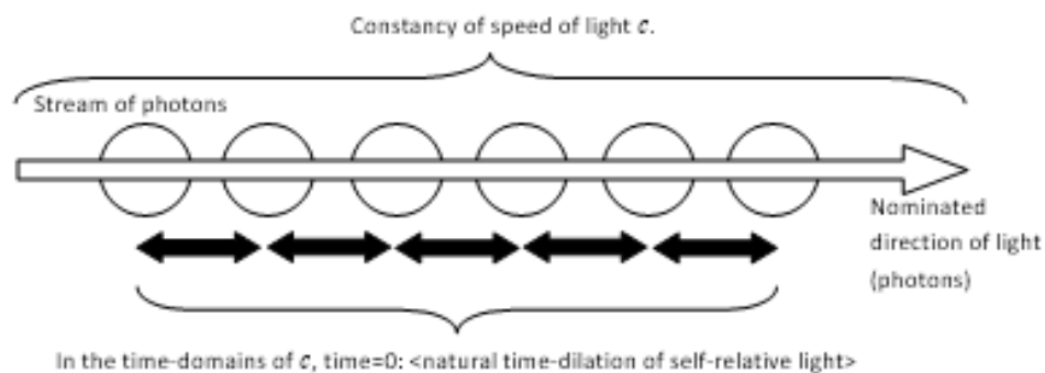
Figure 2: the two fundamental features of light in a vacuum despite relative motion, namely c and how at c time is dilated to the level of time=0.
